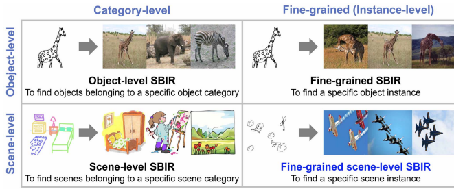
Fig. 1. Illustration of the whole spectrum of SBIR problems. The proposed method, focusing on retrieving the fine-grained scene-level images satisfying the user’s specific requirements via a freehand sketch, is in stark contrast to those of object-level SBIR methods [1], [2] and those focusing on retrieving scene-level images of the same scene class [3].
