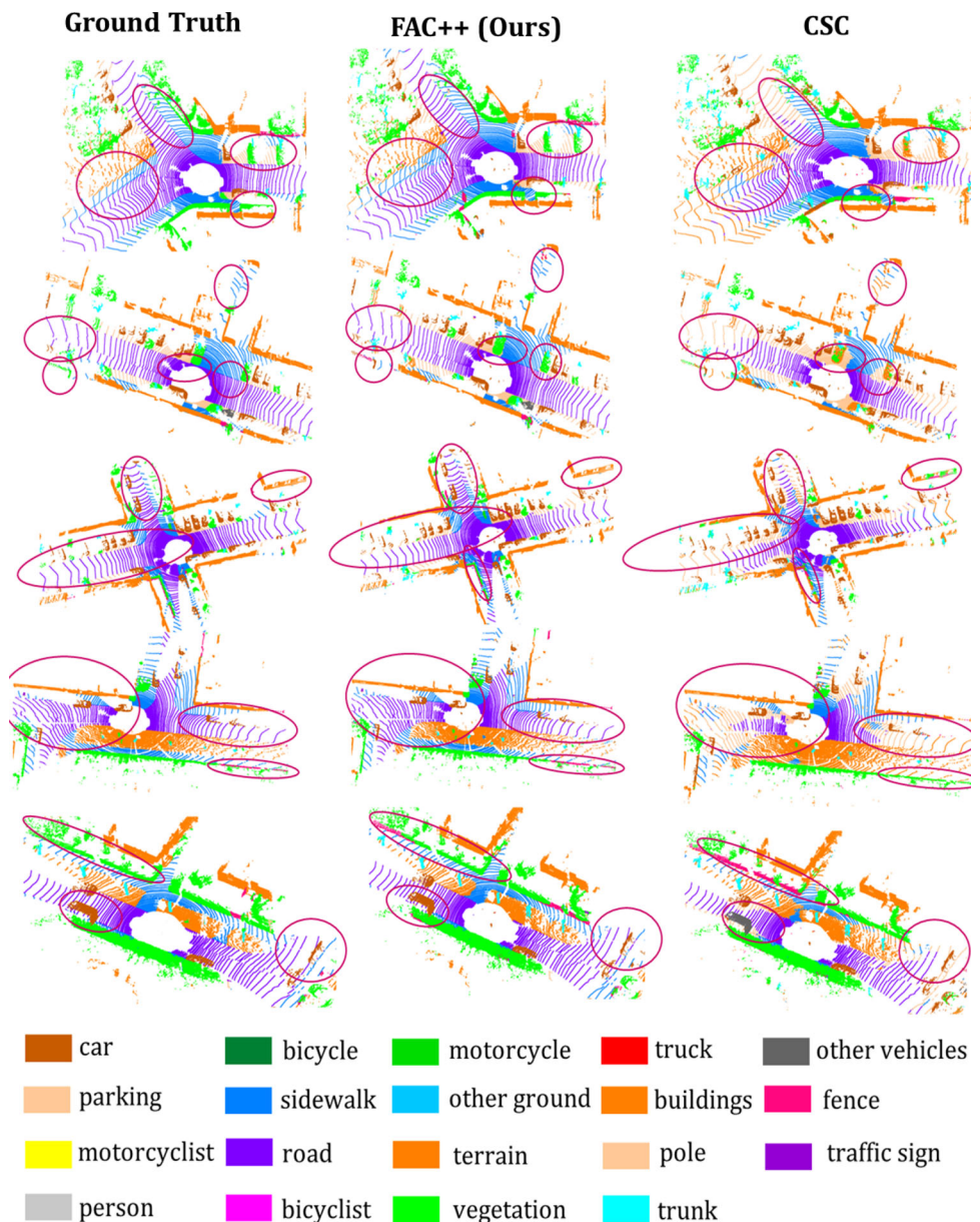
Fig. 11 Comparisons of outdoor 3D Semantic Segmentation Results on SemanticKITTI (Behley et al., 2019) benchmark fine-tuned with 10% labeled training data (ScanNet Dai et al. 2017 pre-trained). Note that the SemanticKITTI (Behley et al., 2019) has no color channel as input for the task of semantic segmentation. Therefore, we visualize the ground truth without visualizing the original scene (no color channel). Differences in prediction are highlighted by the red ellipses
