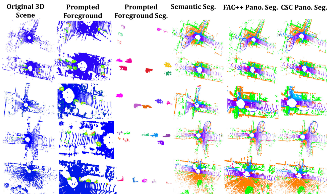
Fig. 4 Visualizations of the outdoor panoptic segmentation in SemanticKITTI. It is demonstrated that our proposed language queries can provide explicit foreground regional information, and the final
