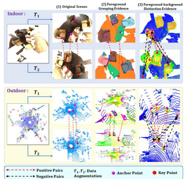
Fig. 1 FAC++ takes both the foreground grouping and the foreground-background distinction guidance into account, thus forming better contrast pairs to learn more informative and discriminative 3D feature representations. FAC++ provides more language-aware information with the 3D visual-linguistic aligned prompts
