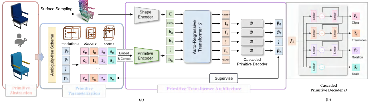
Fig. 2. Overview. We propose PrimitiveAnything to decompose complex shapes into 3D primitive assembly via the auto-regressive transformer. Given human-crafted 3D primitive abstraction contents, we first design an ambiguity-free scheme to parameterize each primitive p into class label c , translation t , rotation r and scale s , and then employ a primitive encoder to form primitive token h . Meanwhile, a shape encoder encodes 3D shape features C from sampled point clouds. Our primitive transformer S predicts the next primitive based on the input condition C and previously generated primitives. To model the dependencies among primitive attributes, we proposed a cascaded primitive decoder \mathcal{D} that sequentially predicts primitive attributes.
