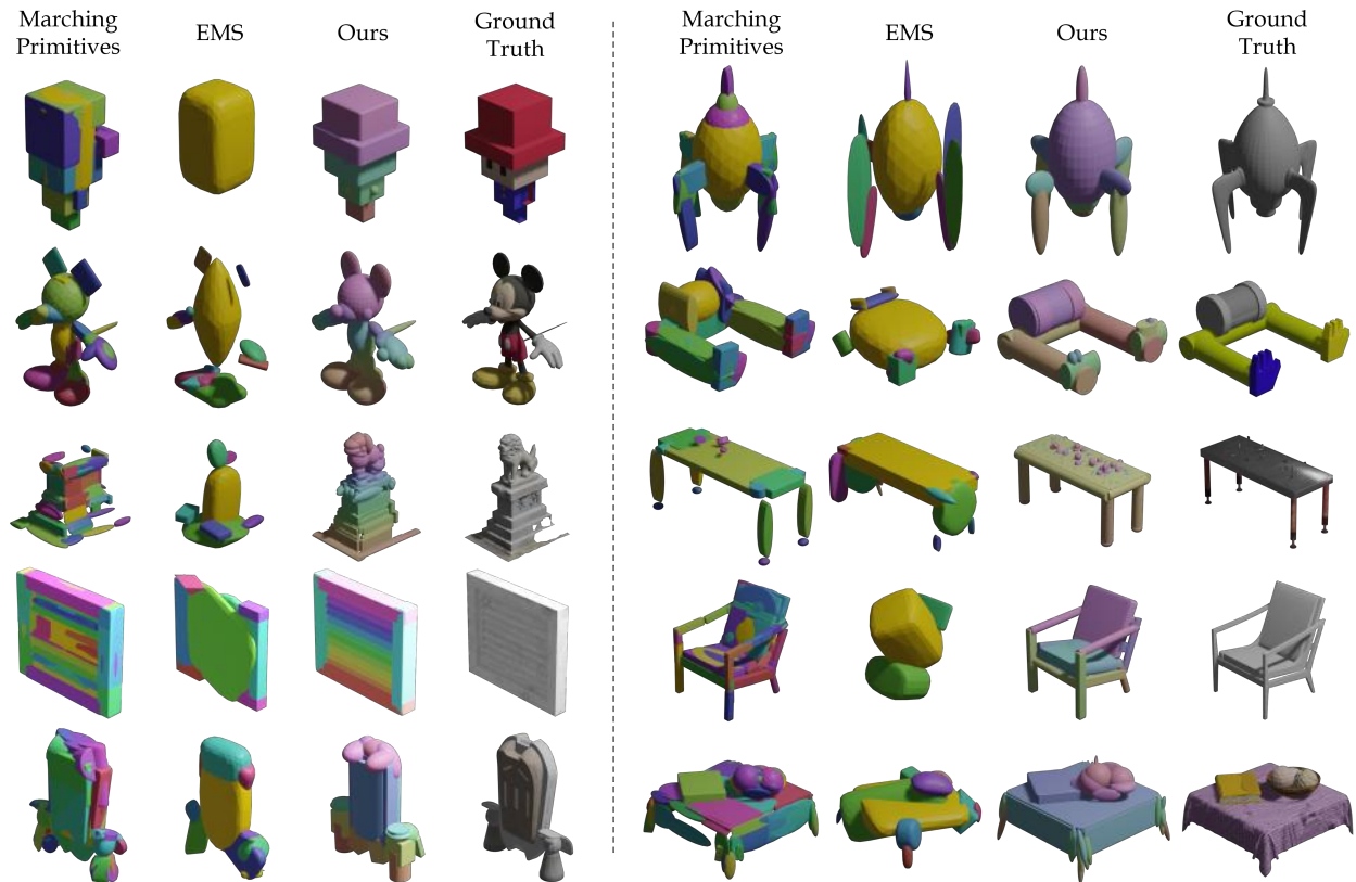
Fig. 9. Comparisons on the Objaverse dataset.
