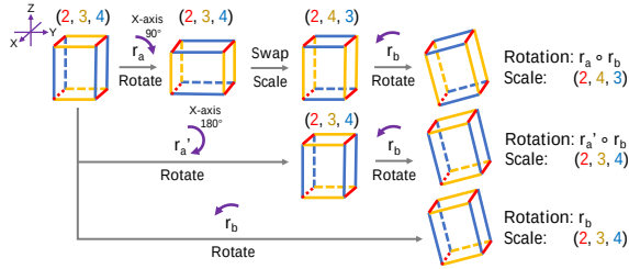
Fig. 3. Demonstration of primitive attribute ambiguity. A primitive with inherent symmetry can correspond to multiple scales and rotations through self-rotation and possible axis swapping.
