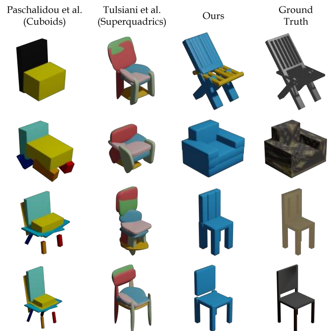
Fig. 8. Comparisons on the ShapeNet test set (Chair category).
