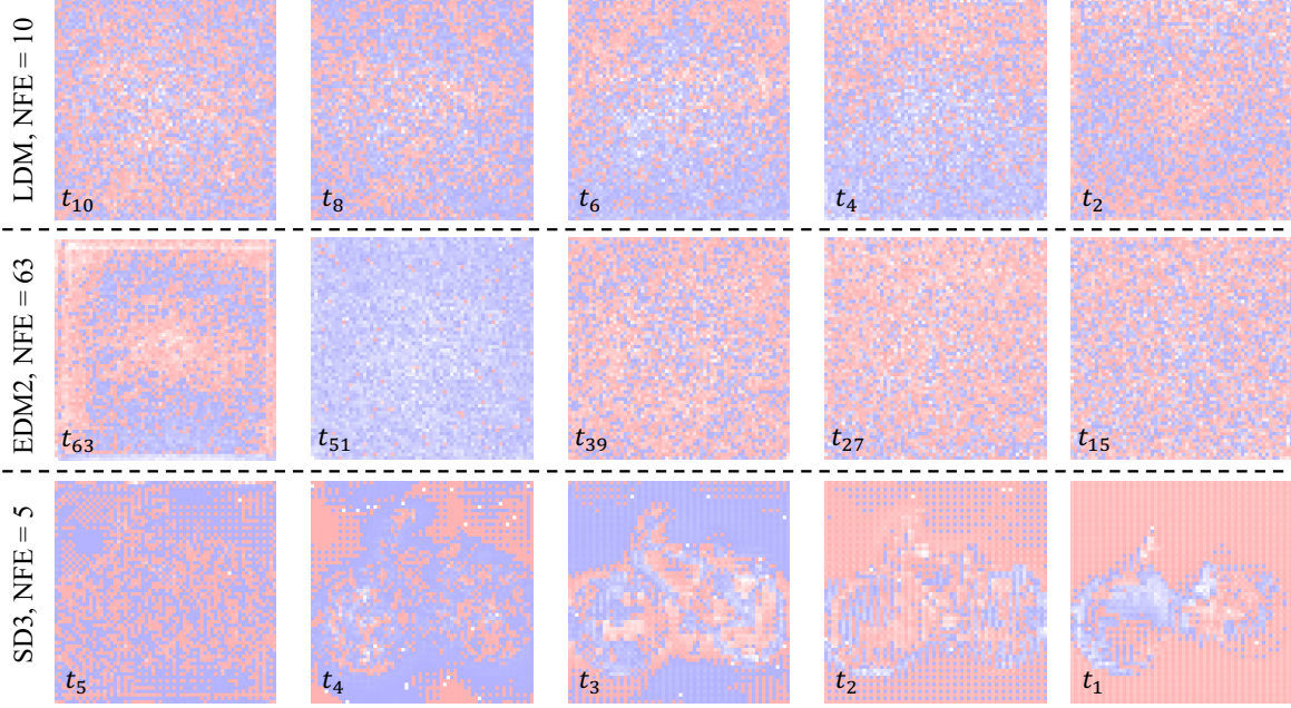
Figure 2. Visualization of the lookup table on LDM [25], EDM2 [16], and SD3 [9], each of which consists of the expectation ratio \mathbb{E}_{\mathbf{x}_t}[\epsilon_\theta(\mathbf{x}_t, c, t)]/\mathbb{E}_{\mathbf{x}_t}[\epsilon_\theta(\mathbf{x}_t, t)] . Each pixel represents the scale of the pixel-wise ratio, i.e. , color red implies that ratio is greater than one, while color blue stands for ratio smaller than one. The darker the color is, the farther the ratio appears away from one. We report in each row the expectation ratios on five timesteps uniformly sampled from the whole trajectory, under different DPMs and NFEs. It is noteworthy that expectation ratios at the same timestep vary largely by different pixels, and there is no general pattern along with timesteps or pixels.
