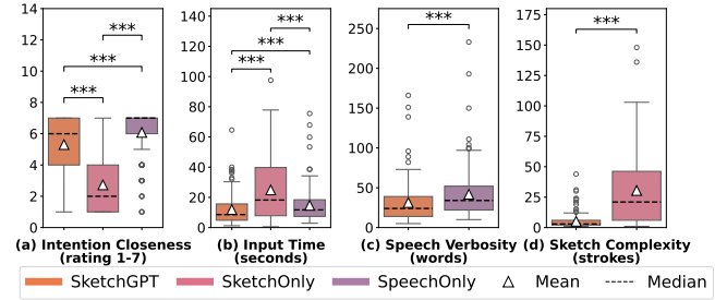
Figure 5: Interaction performance measures from Evaluation Study, Session 1. The X-axis includes three input interfaces: SketchGPT and its baselines, SketchOnly and SpeechOnly. (* indicates p < 0.05 , ** indicates p < 0.01 , *** indicates p < 0.001 )
