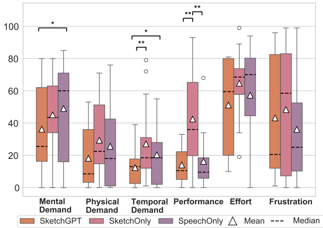
Figure 6: Task load results in NASA-TLX from Evaluation Study, Session1 (the lower the better). The G-axis displays the six NASA-TLX subscales. The Y-axis shows the corresponding scores. (* indicates p < 0.05 , ** indicates p < 0.01 , *** indicates p < 0.001 )
