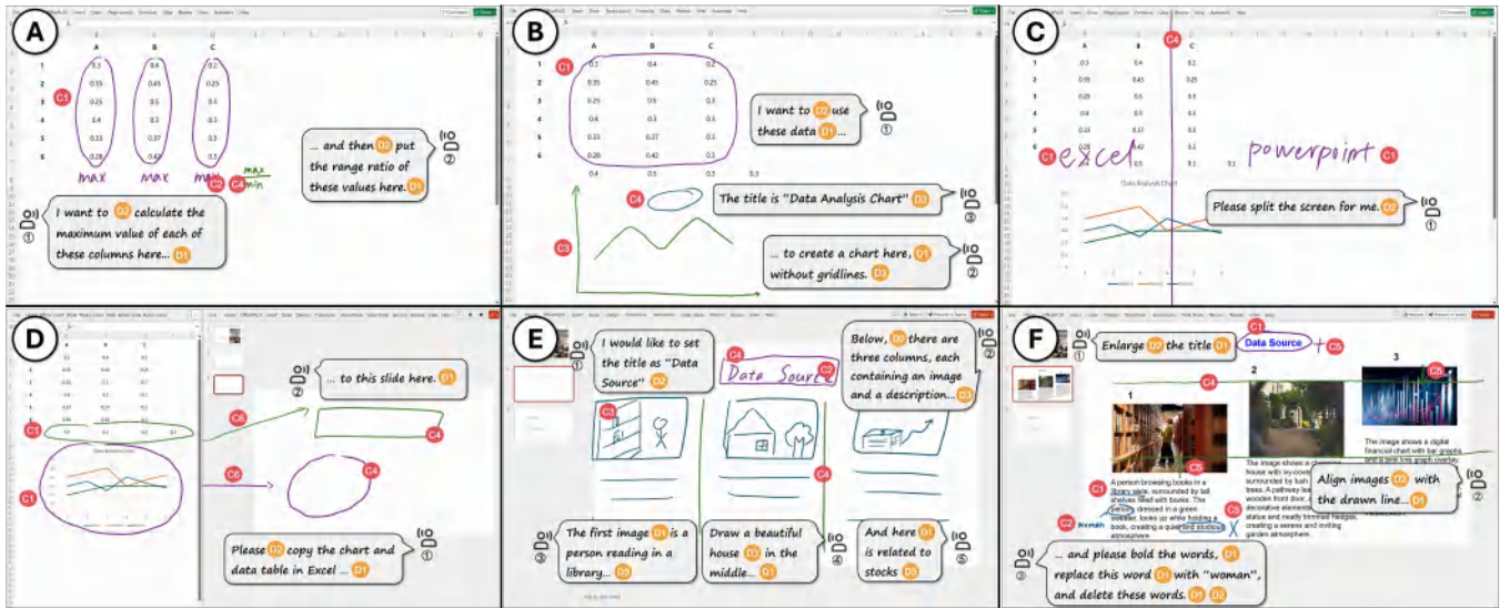
Figure 3: We present an illustrative usagescenario, with the text inside the dialogue box representing user's speechinput: (A) User circles data, inputs formulas, while specifying result placement via speech. (B) User sketches a chart and re nes contents with speech. (C) Texts and symbols are used to convey split-screen operation and position. (D) Circles and arrows indicate cross-app transfer. (E) User sketches the layout and graphics with speechproviding details. (F) Symbolic sketches are used to indicate layout adjustments and content edits.
