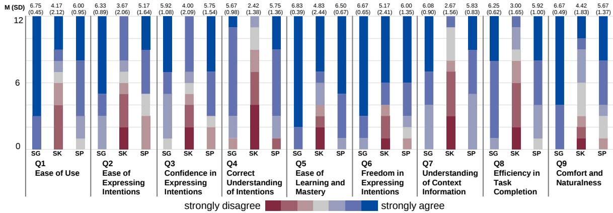
Figure 7: Questionnaire Results on the 7-Point Likert Scale from "Strongly Disagree" to "Strongly Agree" in Evaluation Study, Session1. The X-axis represents different questions, covering various aspects such as system usability evaluation, intention expression, context understanding, and interaction experience. The Y-axis shows the Likert scale ratings provided by participants for different systems across the various questions. SG, SK and SP respectively represent SketchGPT, SketchOnly and SpeechOnly.
